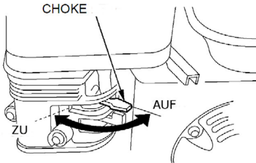
Abb. 7: Choke
